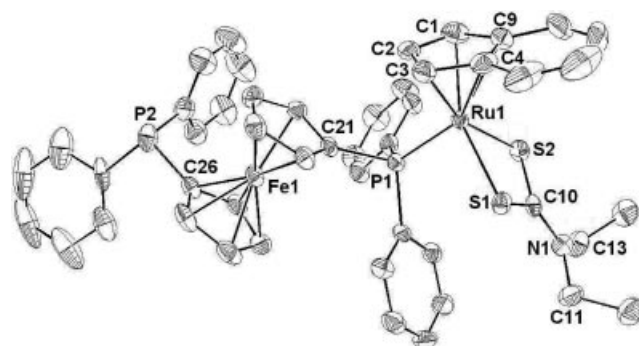
Figure 1. ORTEP diagram of 4a . Thermal ellipsoids are drawn to 50% probability level. Hydrogen atoms are omitted for clarity. Selected bond lengths [ \text{\AA} ] and angles [ ^\circ ]: \text{Ru1-C}^* 1.873 , \text{Ru1-C1 } 2.180(5) , \text{Ru1-C2 } 2.159(5) , \text{Ru1-C3 } 2.185(5) , \text{Ru1-C4 } 2.309(5) , \text{Ru1-C9 } 2.302(5) , \text{Ru1-P1 } 2.2392(13) , \text{Ru1-S1 } 2.4068(13) , \text{Ru1-S2 } 2.3826(14) , \text{S1-C10 } 1.699(5) , \text{S2-C10 } 1.718(5) , \text{C10-N1 } 1.337(6) , \text{P1-C21 } 1.825(5) , \text{P2-C26 } 1.810(6) , \text{S1-Ru1-S2 } 71.85(4) , \text{S1-Ru1-P1 } 93.73(5) , \text{S2-Ru1-P1 } 88.04(5) , \text{S1-C10-S2 } 110.7(3) , \text{S1-C10-N1 } 126.3(4) , \text{S2-C10-N1 } 122.9(4) , \text{C10-N1-C11 } 121.1(4) , \text{C10-N1-C13 } 119.7(4) , \text{Ru1-P1-C21 } 111.90(16) .
