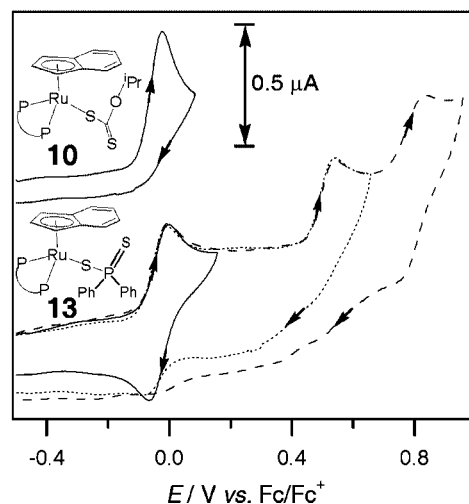
Figure 8. Cyclic voltammograms performed at a 1-mm diameter planar GC electrode in \text{CH}_2\text{Cl}_2 (0.25 M \text{Bu}_4\text{NPF}_6 ) at 233 K at a scan rate of 100 mV/s for 0.5 mM 10 and 13 .
