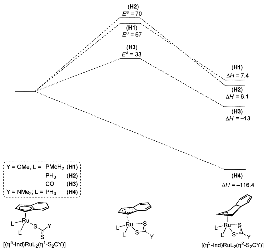
Figure 7. Energy diagram of ring slippage from \eta^5 \rightarrow \eta^3 ( E^a is activation energy in kJ/mol).
