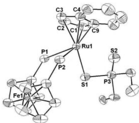
Figure 3. ORTEP diagram of 12 . Thermal ellipsoids are drawn to 50% probability level. Hydrogen atoms and phenyl groups are omitted for clarity. Selected bond lengths [Å] and angles [°]: Ru1–C* 1.941, Ru1–C1 2.244(8), Ru1–C2 2.168(7), Ru1–C3 2.182(7), Ru1–C4 2.408(7), Ru1–C9 2.424(8), Ru1–P1 2.2516(19), Ru1–P2 2.3181(18), Ru1–S1 2.4647(18), P1–Ru1–P2 98.98(7), S1–Ru1–P1 89.27(7), S1–Ru1–P2 86.07(6).
