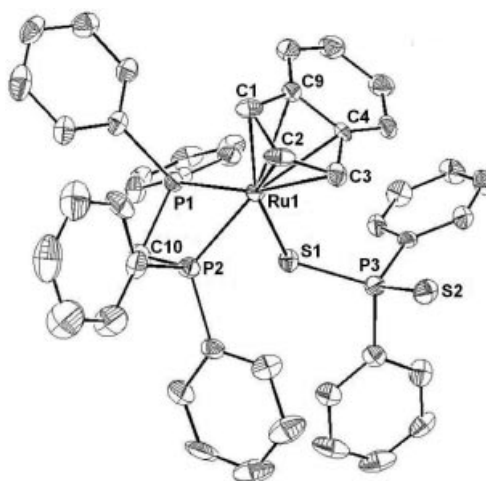
Figure 4. ORTEP diagram of 16 . Thermal ellipsoids are drawn to 50% probability level. Hydrogen atoms are omitted for clarity. Selected bond lengths [Å] and angles [°]: Ru1–C* 1.884, Ru1–C1 2.161(7), Ru1–C2 2.183(7), Ru1–C3 2.223(7), Ru1–C4 2.318(7), Ru1–C9 2.321(7), Ru1–P1 2.2695(19), Ru1–P2 2.242(2), Ru1–S1 2.439(2), S1–P3 2.044(3), S2–P3 1.965(3), C10–P1 1.848(7), C10–P2 1.848(8), P1–Ru1–P2 72.20(7), S1–Ru1–P1 84.98(7), S2–Ru1–P2 84.76(7), Ru1–S1–P3 117.45(10), S1–P3–S2 121.02(14), P1–C10–P2 92.0(3).
