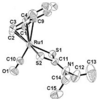
Figure 6. ORTEP drawing of (\text{Ind})\text{Ru}(\text{CO})(\text{S}_2\text{CNEt}_2) 21 with 50% probability thermal ellipsoids. H atoms are omitted for clarity. Selected bond lengths [Å] and angles [°]: Ru1–C* 1.910, Ru1–C1 2.210(4), Ru1–C2 2.174(4), Ru1–C3 2.191(4), Ru1–C4 2.358(4), Ru1–C9 2.372(4), Ru1–S1 2.4035(10), Ru1–S2 2.3930(10), S1–C11 1.712(4), S2–C11 1.724(4), C11–N1 1.320(5), Ru1–C10 1.807(4), S1–Ru1–S2 72.22(3), S1–C11–S2 110.7(2).
