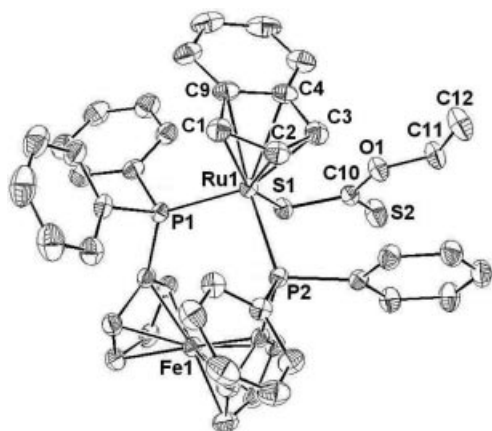
Figure 2. ORTEP diagram of 9 . Thermal ellipsoids are drawn to 50% probability level. Hydrogen atoms are omitted for clarity. Selected bond lengths [Å] and angles [°]: Ru1–C* 1.918, Ru1–C1 2.220(3), Ru1–C2 2.186(3), Ru1–C3 2.212(3), Ru1–C4 2.361(3), Ru1–C9 2.374(3), Ru1–P1 2.3110(7), Ru1–P2 2.2618(7), Ru1–S1 2.3964(7), S1–C10 1.712(3), S2–C10 1.674(3), C10–O1 1.331(4), P1–Ru1–P2 97.43(3), S1–Ru1–P1 89.31(3), S2–Ru1–P2 86.53(3), Ru1–S1–C10 116.03(10), S1–C10–S2 120.60(17), S1–C10–O1 116.4(2), S2–C10–O1 123.0(2), C10–O1–C11 118.5(2).
