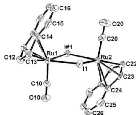
Figure 5. ORTEP drawing of [(\text{Ind})\text{Ru}(\text{CO})\text{I}]_2 20 with 50% probability thermal ellipsoids. H atoms are omitted for clarity. Selected bond lengths [Å] and angles [°]: Ru1–C* 1.874, Ru1–C12 2.142(16), Ru1–C13 2.172(10), Ru1–C14 2.334(10), Ru2–C* 1.885, Ru2–C22 2.141(15), Ru2–C23 2.171(10), Ru2–C24 2.356(10), Ru1...Ru2 4.014, Ru1–I1 2.716(10), Ru2–I1 2.717(10), Ru1–C10 1.820(15), Ru2–C20 1.812(16), I1–Ru1–I#1 84.37(4), I1–Ru2–I#1 84.35(4), C10–Ru1–I1 93.1(4), C20–Ru2–I1 92.5(4), Ru1–I1–Ru2 95.26(3).
